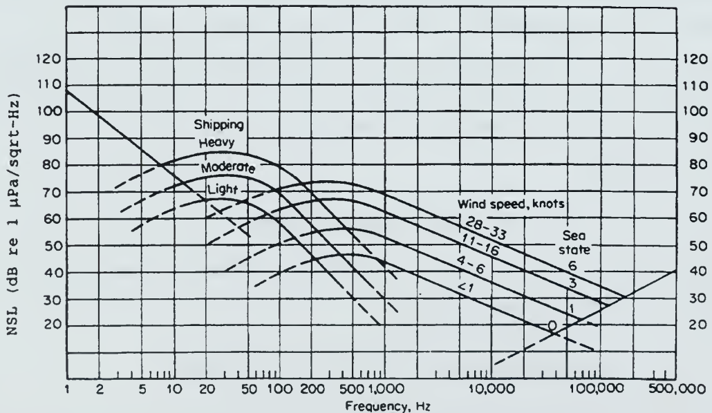
Figure 2.1. Average deep-water ambient noise spectral density levels [2].
